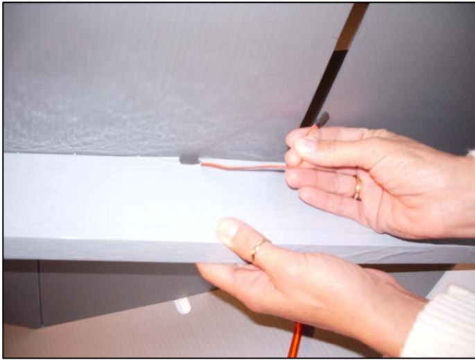
Servo wire exits on inside of nacelle.
